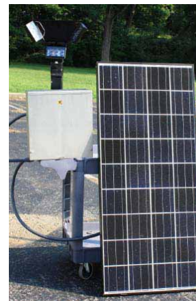
SL-45 WITH SOLAR OPTION
